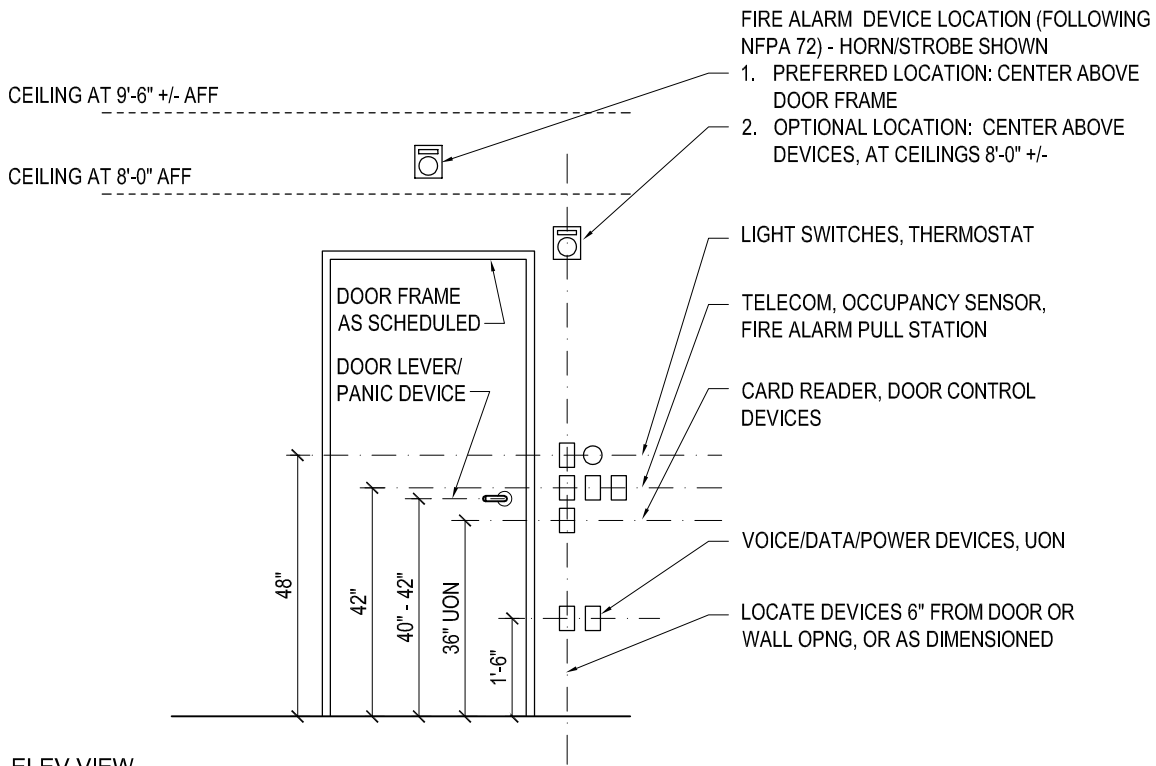
ELEV VIEW
